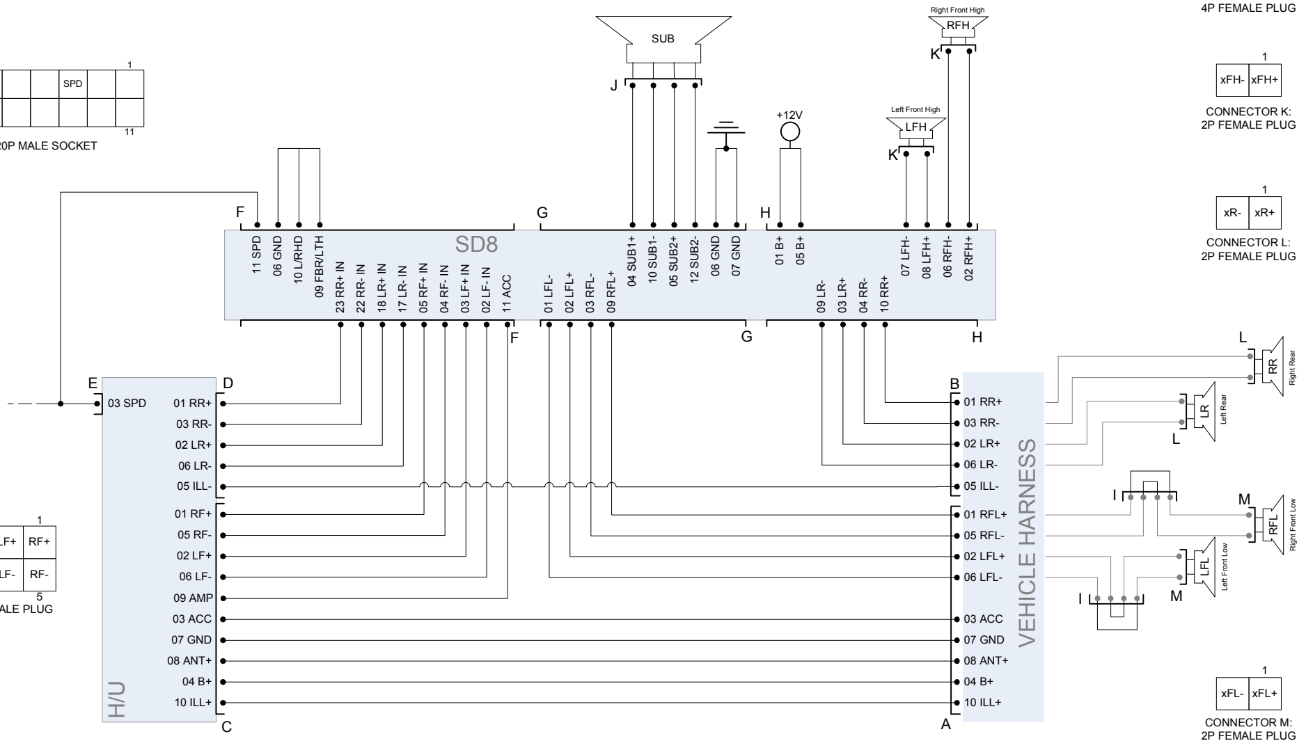
CONNECTOR G: 12P FEMALE PLUG
