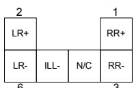
CONNECTOR B: 6P MALE SOCKET
