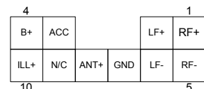
CONNECTOR A: 10P MALE SOCKET
