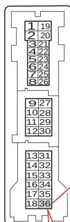
"WIRE VIEW"
